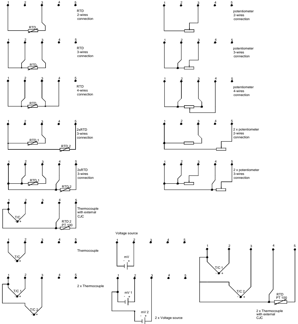
Fig.7. Sensors connection options to LI-24 transmitter.
