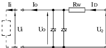
Fig.3. The supplying principle with a source of trapezoidal characteristics.
