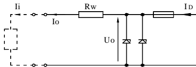
Fig. 2. The supplying principle with a source of linear characteristics
